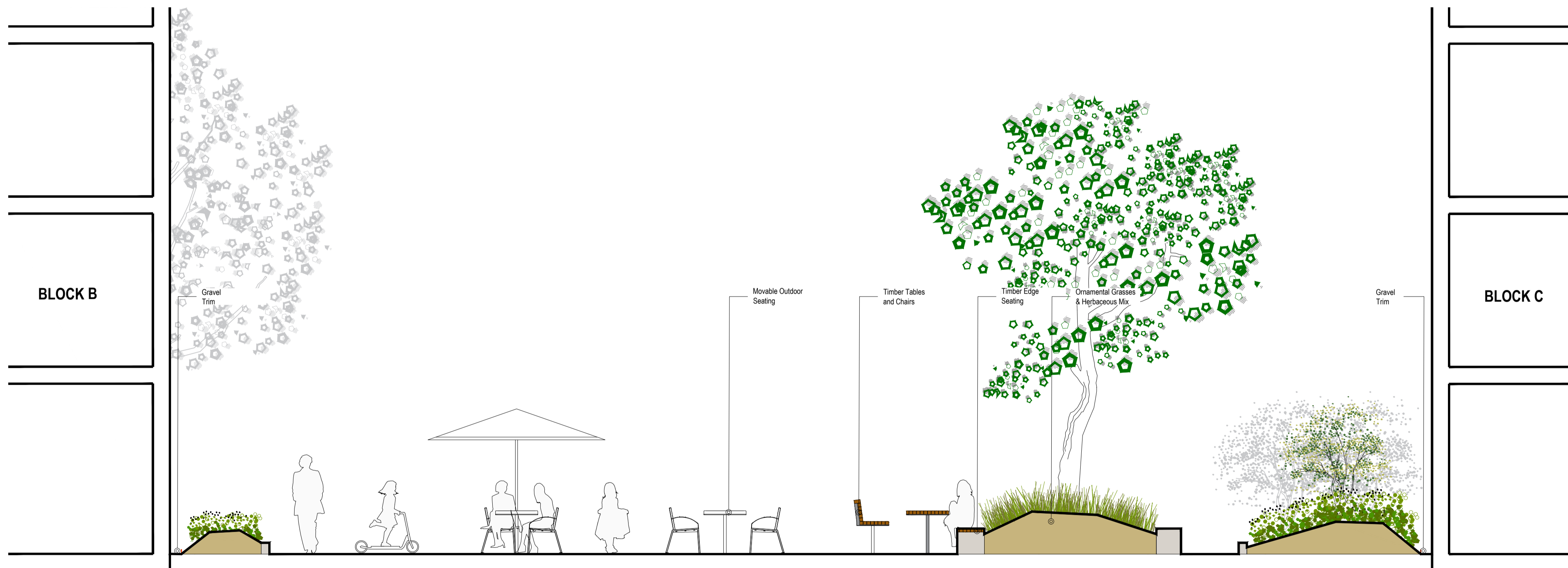
D-D Central Courtyard Scale 1:50
